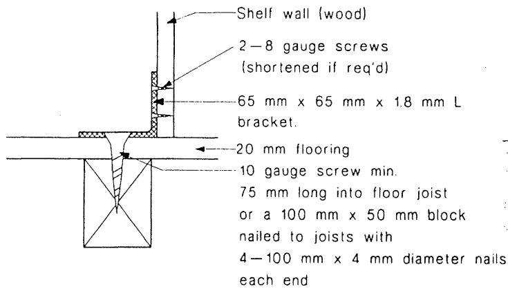
DETAIL A - TIMBER FLOOR
