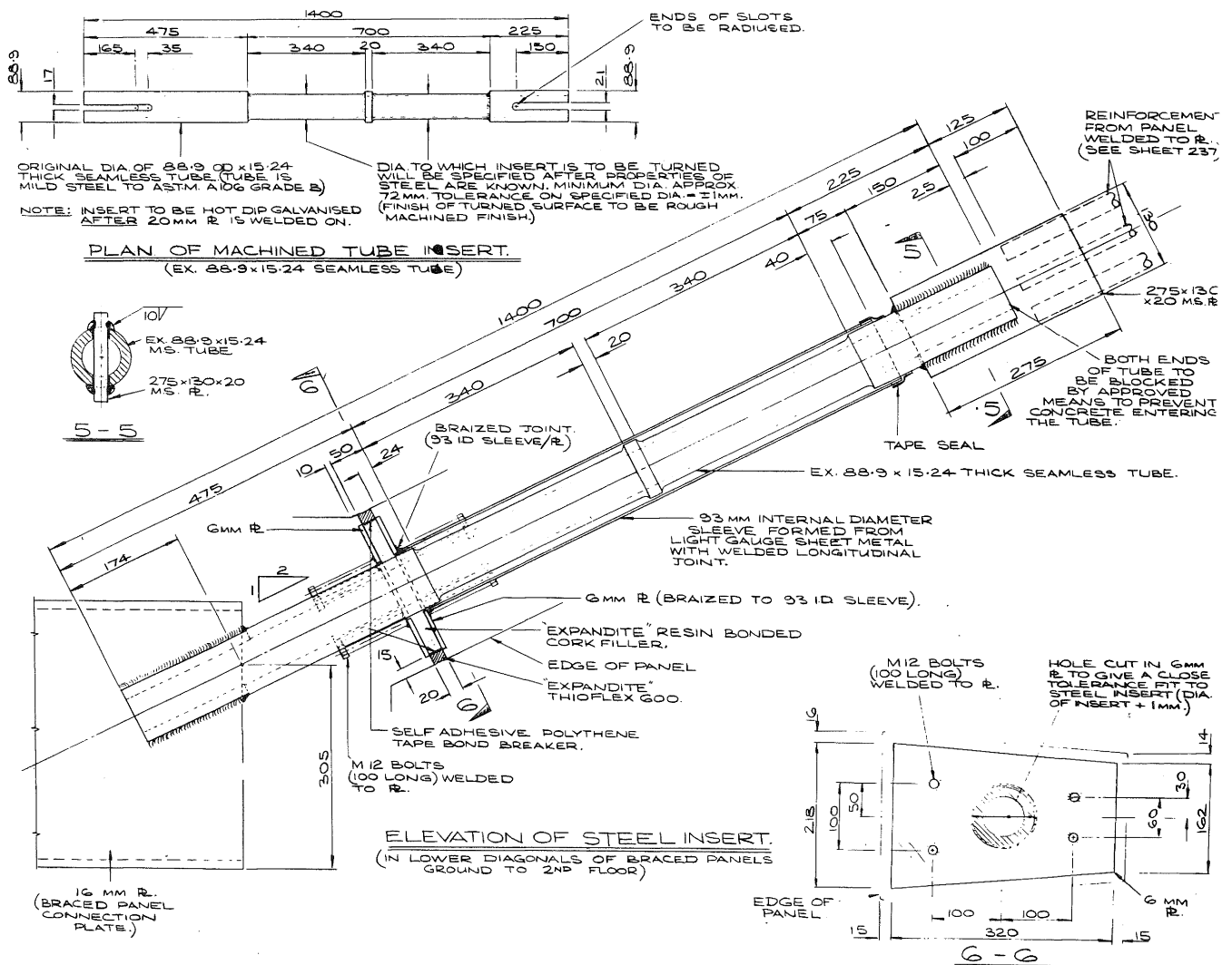
Figure 6. Revised Steel Insert Details
