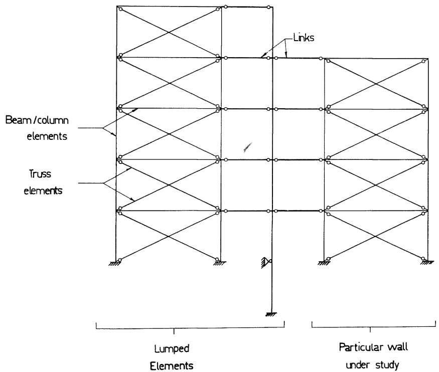
Figure 3. Dynamic Analysis Model
