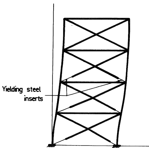
Figure 2. Typical deflected shape of typical wall under seismic load
