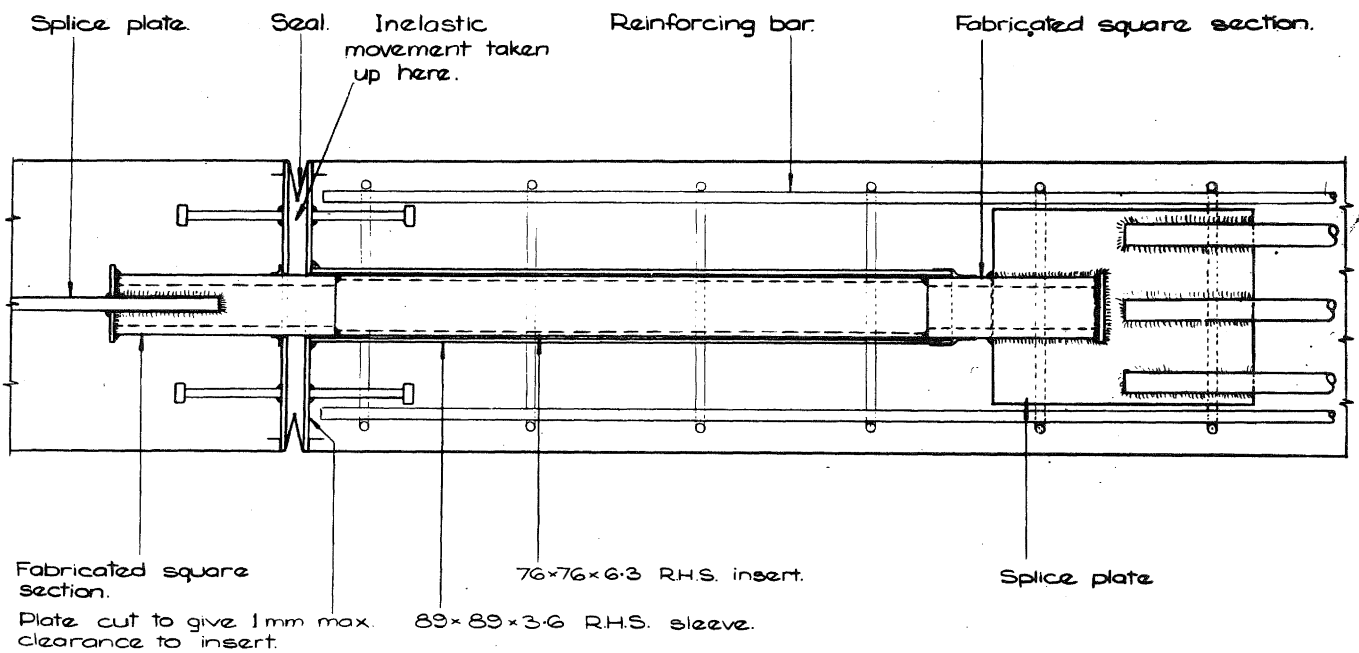
Figure 5. Steel Insert Details
