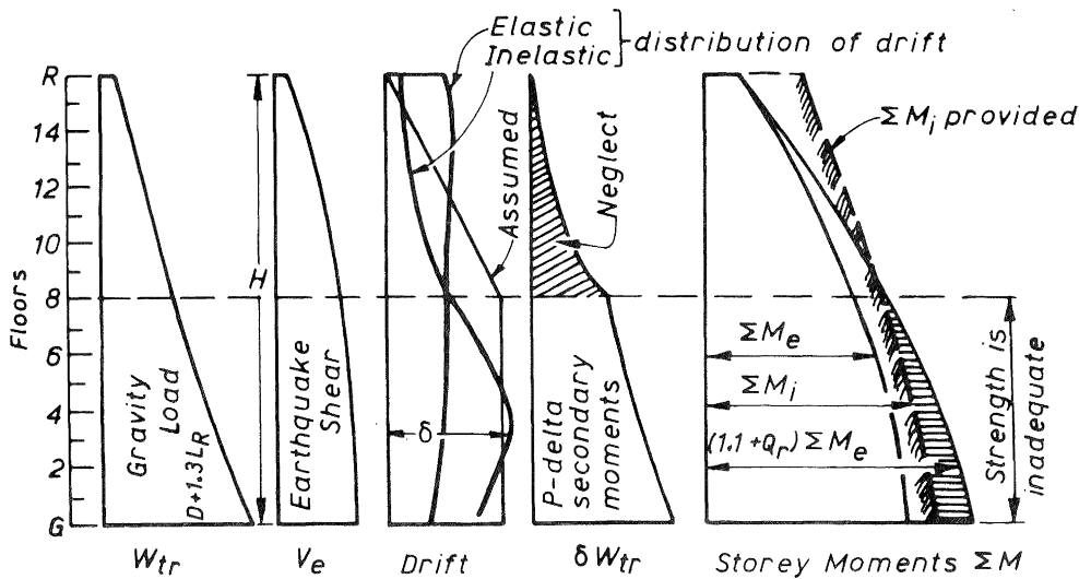
FIGURE 8: SOME DESIGN QUANTITIES FOR A 16 STOREY DUCTILE FRAME
