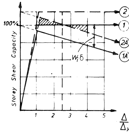
FIGURE 6: IDEALISED BILINEAR RESPONSES ALSO SHOWING THE EFFECT OF P-DELTA MOMENTS
