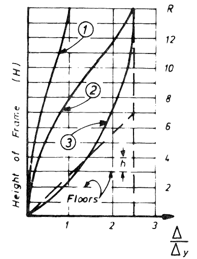
FIGURE 7: A COMPARISON OF DEFLECTED SHAPES OF ELASTIC AND IN ELASTIC FRAMES
