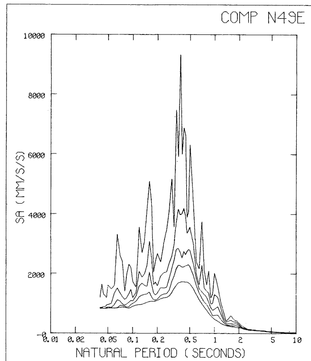
FIGURE 6: (b) CORRESPONDING RESPONSE SPECTRA FOR ACCELERATION COMPONENT, N49°E.
