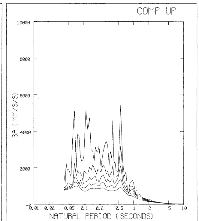
FIGURE 6: (c) CORRESPONDING RESPONSE SPECTRA FOR ACCELERATION COMPONENT, UPWARDS
