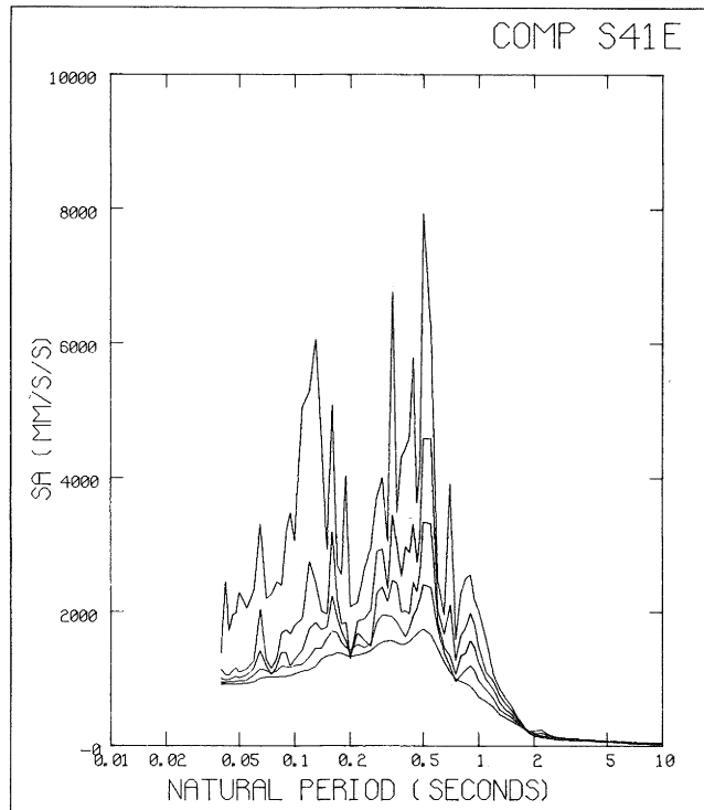
FIGURE 6: (a) ACCELERATION RESPONSE SPECTRA FOR ACCELERATION COMPONENT S41°E, FOR RESONATORS WITH 0, 2%, 5%, 10%, 20% OF CRITICAL DAMPING
