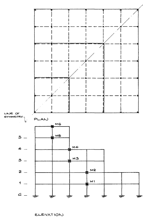
FIGURE 4: BUILDING 4 (IRREGULAR, MODERATE TO HIGH ECCENTRICITY. 3D MODAL ANALYSIS)
