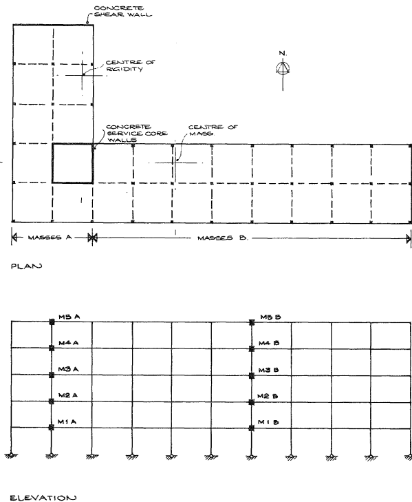
FIGURE 7: BUILDING 7 (REGULAR, MODERATE ECCENTRICITY EAST-WEST, HIGH ECCENTRICITY IN NORTH-SOUTH. 3D MODAL ANALYSIS IS RECOMMENDED)
