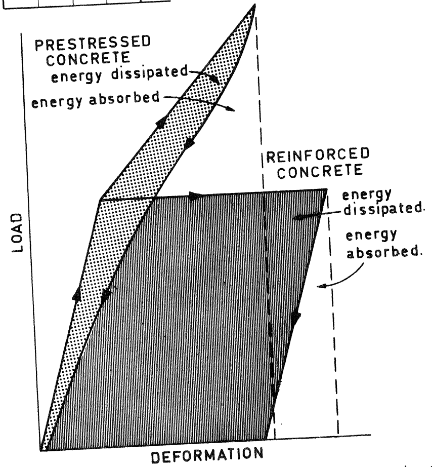
FIG. 5. Dissipation of energy in PSC and RC members, after Candy 12 .
