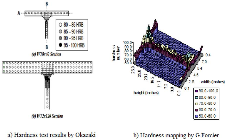
Figure 8: Hardness test results by Okazaki in 2004 [17] and G.Forcier [18, 19].
