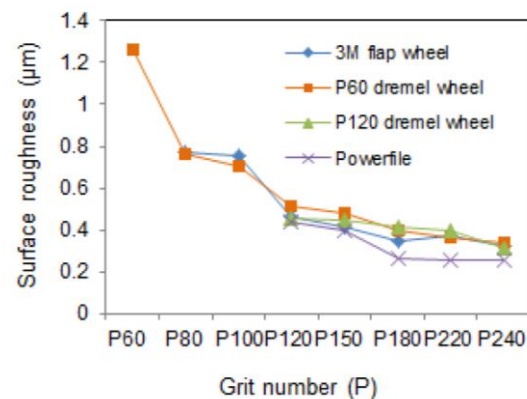
Figure 2: Comparison of surface roughness with different surface cleaning methods [9].
