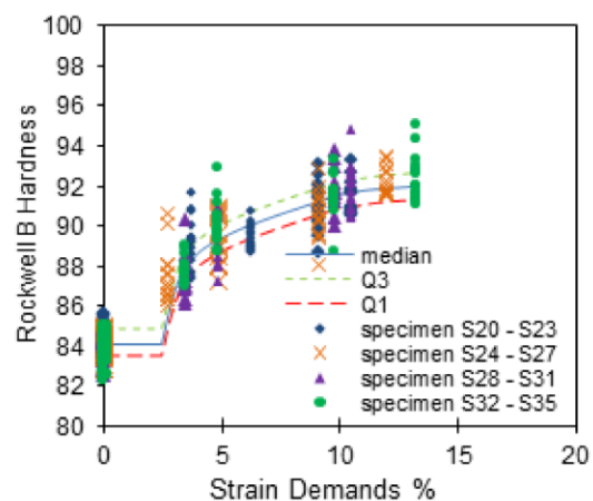
(b) Tensile-hardness relationship for 12mm thick specimens
