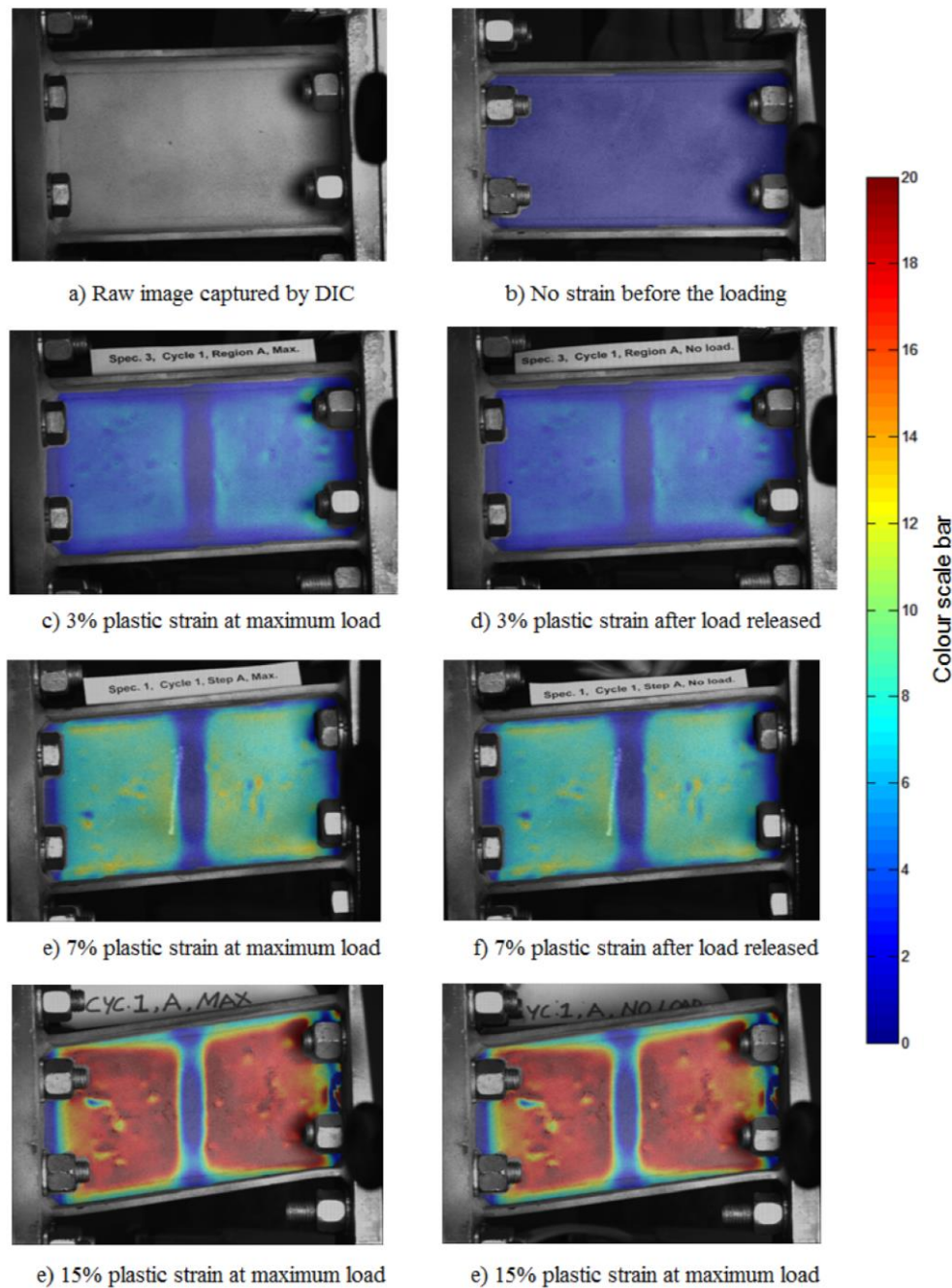
Figure 10: Strain contour plots across the web of the active link specimens using DIC by CACM at The University of Auckland.
