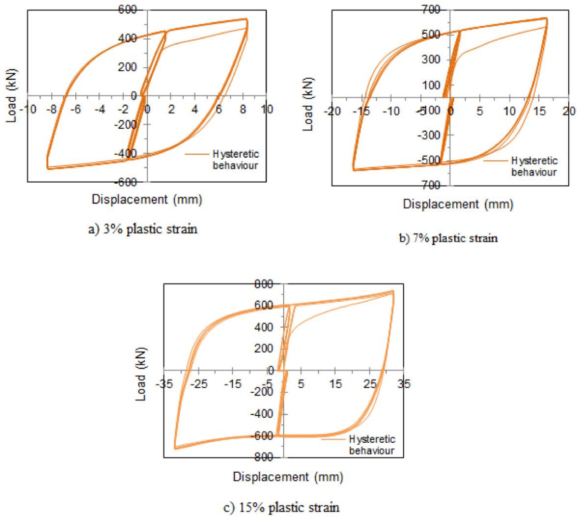
Figure 6: Cyclic load displacement behaviour.
