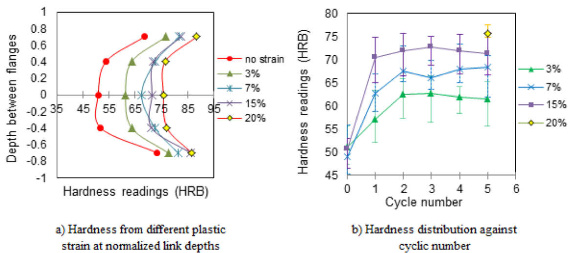
Figure 7: Comparison of average hardness from the five cycles of loading with different cyclic plastic strain levels using TH170 and hardness comparison at the centre of the link versus cyclic number for different strain levels.
