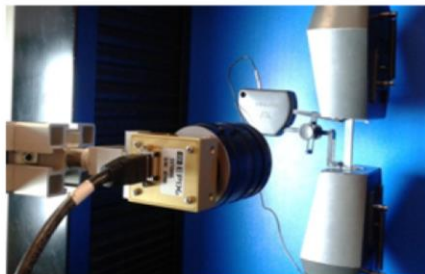
a) DIC test setup for monotonically loaded specimen
