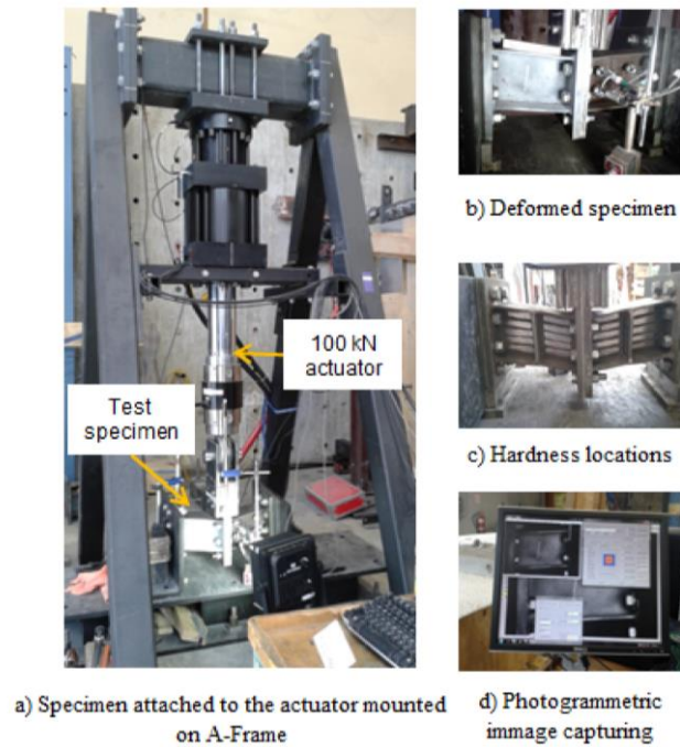
Figure 5: A full scale active link specimen under cyclic loading. Test Hall, University of Auckland.
