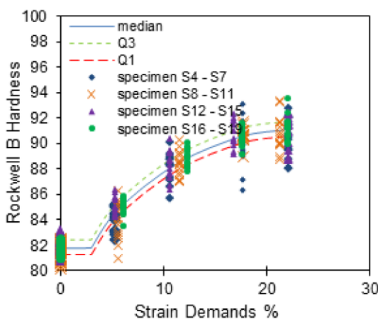
(a) Tensile-hardness relationship for 8mm thick specimens
