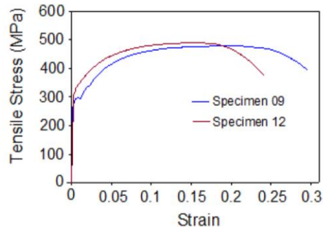
b) Overall DIC stress vs strain curves
