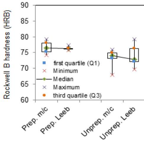
Figure 3: Comparison of hardness between surfaces prepared to R_a < 0.6 microns and unprepared surfaces using a Rockwell B machine and Leeb TH170 hardness tester on a 25 mm thick specimen.
