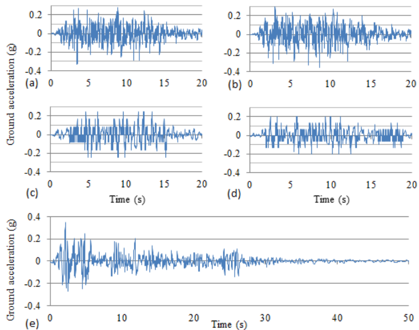
Figure 4: Ground motions (a) NZDS 1, (b) NZDS 2, (c) JDS 1, (d) JDS 2 and (e) El C.
