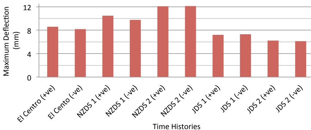
Figure 5: Maximum deflection of the reference frame under time histories considered without pounding effect.
