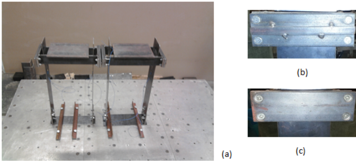
Figure 3: Adjacent structure without seismic gap: (a) Frames on shake table, and pounding interface on, (b) left frame and (c) right frame.
