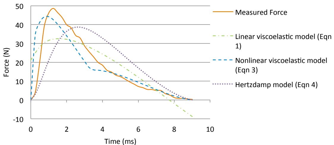
Figure 7: Measured force time history and numerical approximations.
