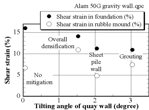
Figure 26: Shear deformation in foundation and rubble mound.
