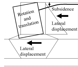
Figure 11: Typical configuration of quay wall distortion.
