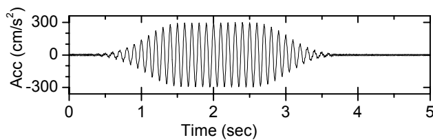
Figure 16: Time history of base shaking.
