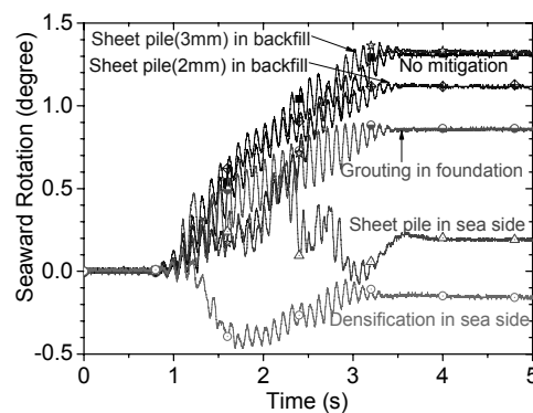
Figure 18: Time history of rotation of quay wall.
