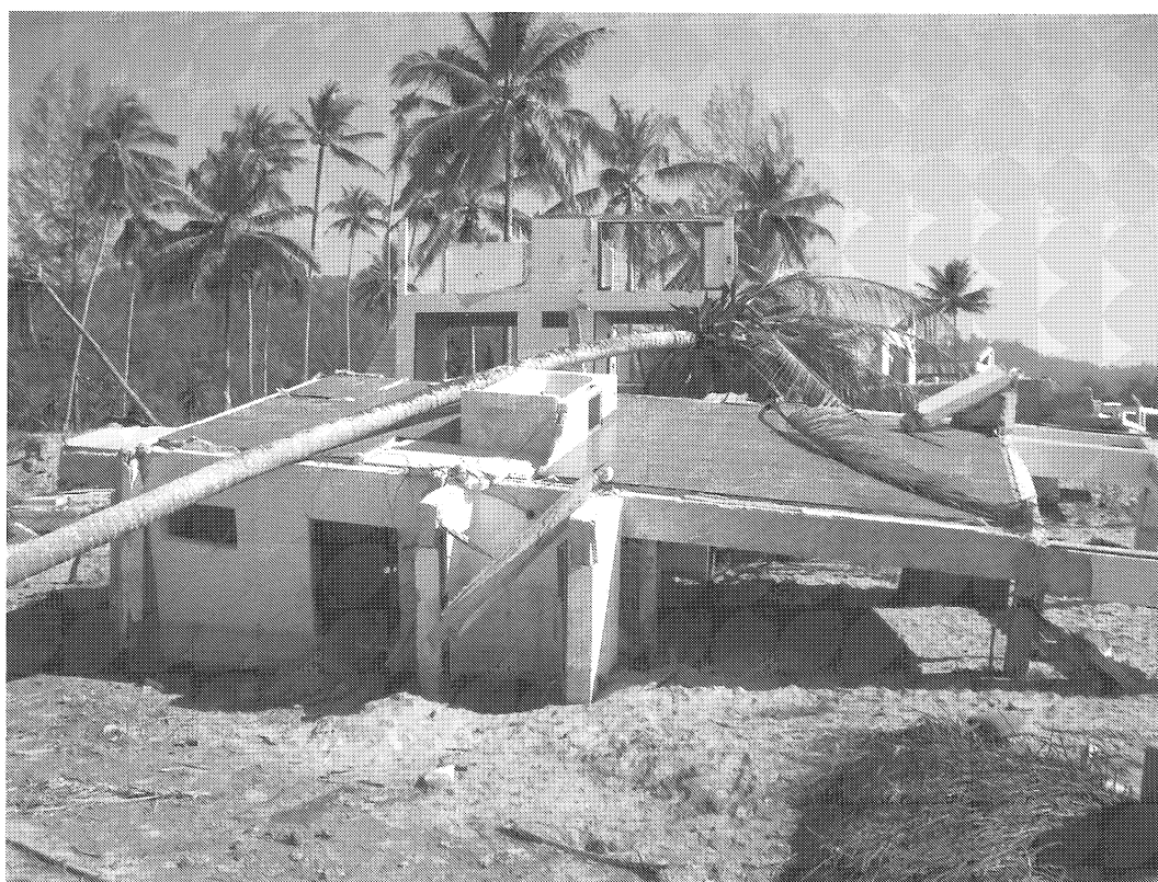
Figure 15a and 15b. The receding waters after each wave caused substantial scouring of small streams and low-lying depressions, as shown here at Khao Lak. The scoured “channel” (15a) is 50 m wide and up to 3 m deep, completely undermining the resort buildings (15b) nearby (Photos RB).
