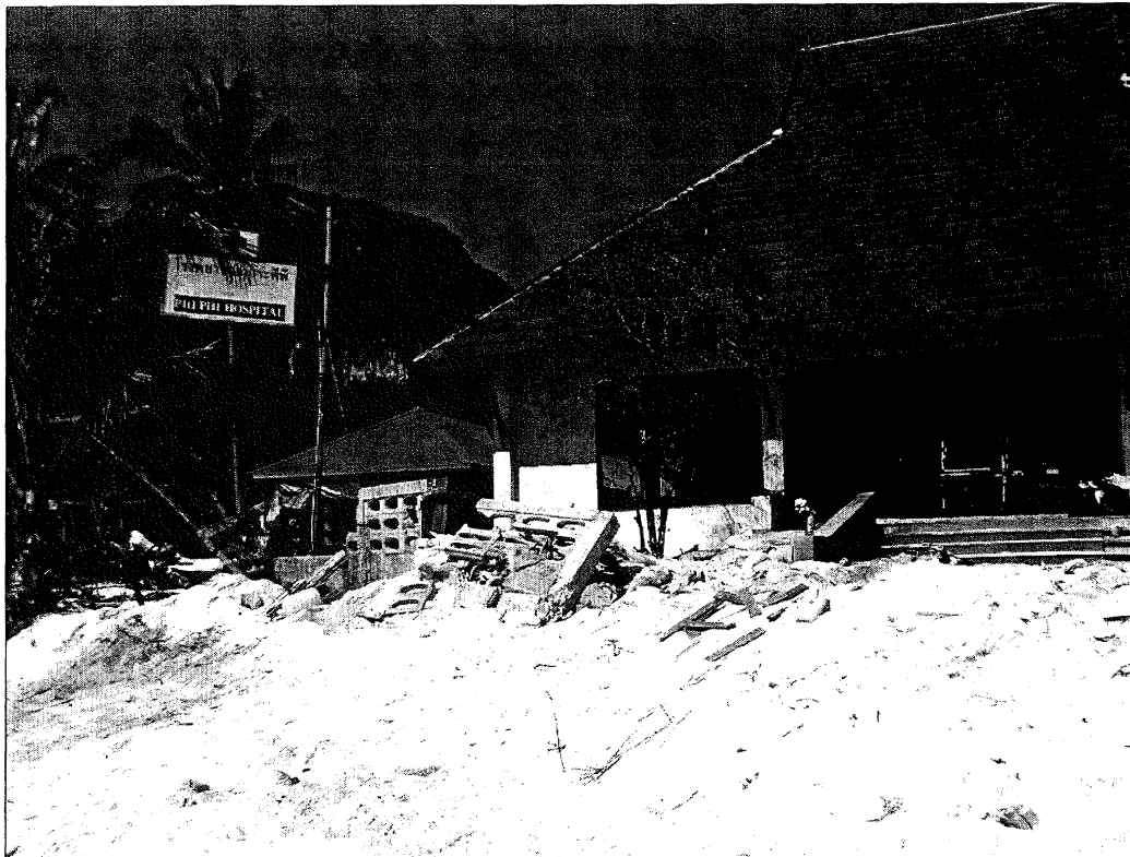
Figure 8. The hospital on Koh Phi Phi was set back from the shore but situated close to sea-level. It was rendered inoperable by the tsunami, highlighting the critical need to locate such facilities outside potential inundation zones (Photo LY).
