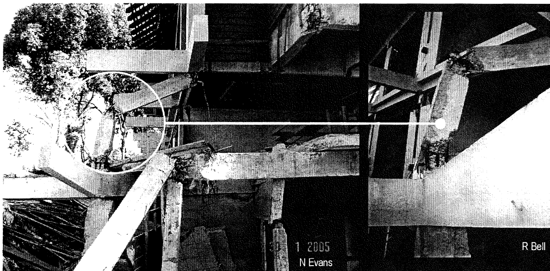
Figure 12. Damage to reinforced concrete frame structures was only locally severe, where exposed structural elements were impacted by entrained debris (Photos NE and RB).
