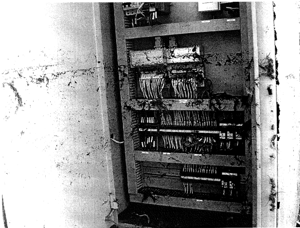
Figure 9a and 9b. Inspecting damage to a sewerage pumping station at Kata Beach, Phuket Island. Electrical control systems were damaged beyond repair, causing sewer overflows into the adjacent stream, and discharge onto the nearby beach (Photos RB and HC).
