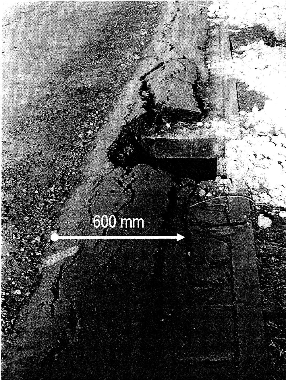
Figure 10. Damage to roads was locally severe due to scouring. At Kamala Beach, Phuket Island, where the torrent depth was 3-4 m, the beach-front road pavement was shifted landward 600 mm onto the adjacent stormwater drain cover.
