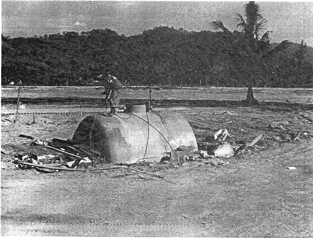
Figure 16. Liquefaction of soils appears to have occurred during the surge and withdrawal of tsunami waters at Khao Lak, with underground services such as this tank floating to the surface (Photo NE).
