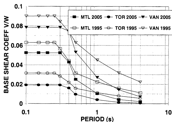
Figure 5. Conventional Construction Steel Moment Frame on Hard Rock.
