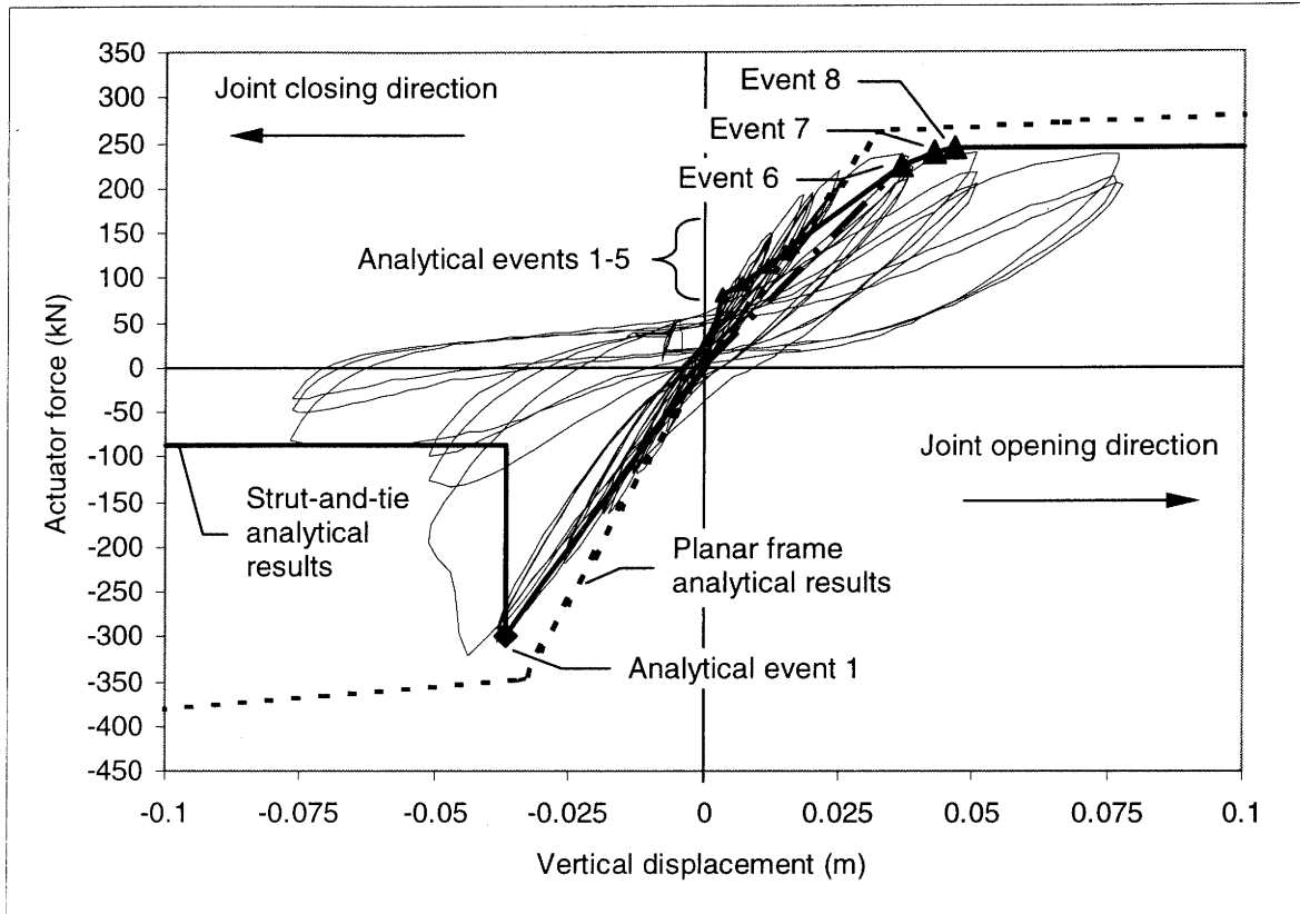
a) As-built knee-joint vertical displacement history.
