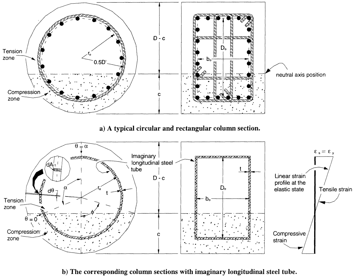
Figure 4. Circular and rectangular column sections.
