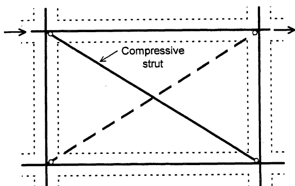
Figure 1: Diagonal strut model for infilled frames.
