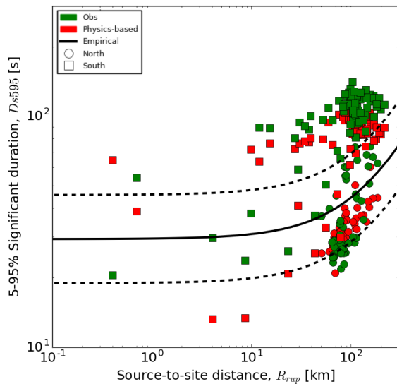
Figure 8: Observed, simulated, and empirically-predicted 5-95% Significant Duration ( D_{S595} ) as a function of source-to-site distance, R_{rup} . Symbol shape indicates location of the station in the North or South Island. The median, and 16 th /84 th percentiles of the empirical prediction [26] are represented by solid and dashed lines, respectively (based on a reference V_{s30} = 250\text{m/s} condition).
