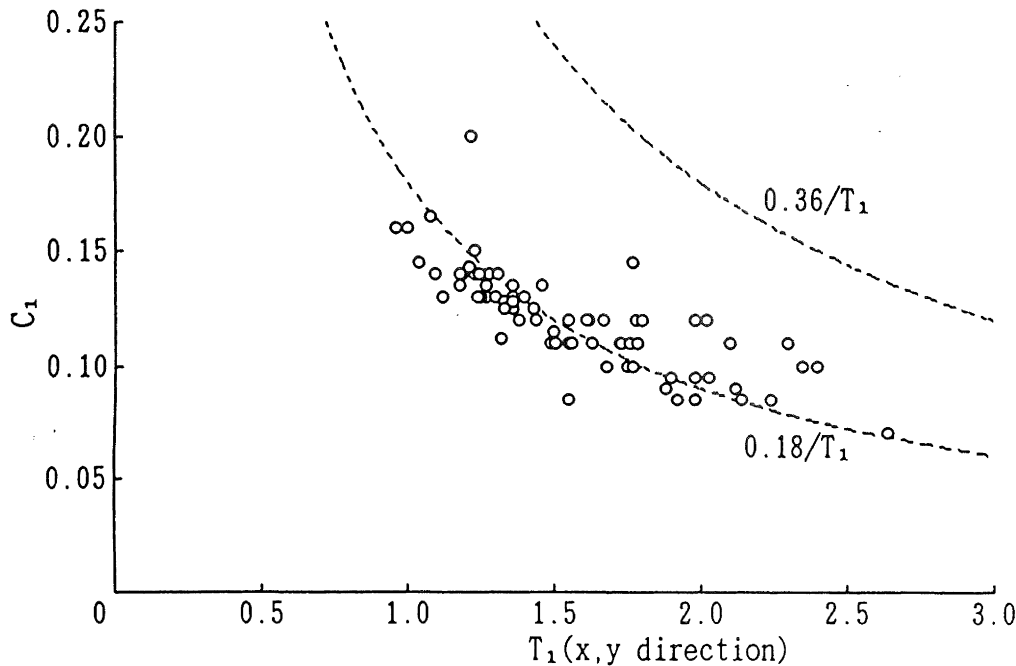
(b) Fundamental period from analysis
