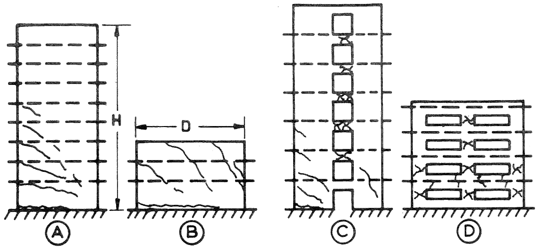
Fig. 4. Types of Regular Shear Walls in Multistorey Buildings.
