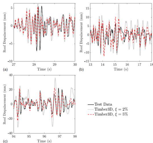
Figure 35: Displacement response of test results and models using 2% and 5% damping [42] under earthquake records of (a) Darfield 2010, (b) Lyttelton 2011, (c) Kaikōura 2016.
