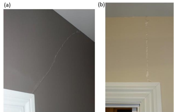
Figure 36: Plasterboard bracing walls damage after the 2010 Darfield earthquake: (a) diagonal cracking of plasterboard; (b) vertical cracking of plasterboard [8].
