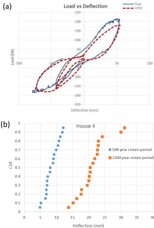
Figure 31: Single-degree of freedom nonlinear model based on HYST model for a case study building [40]: (a) hysteresis curves; and (b) cumulative distribution of peak displacement responses.
