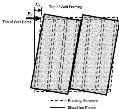
Figure 22: Assumption of racking mode for wood-framed shear walls [27].
