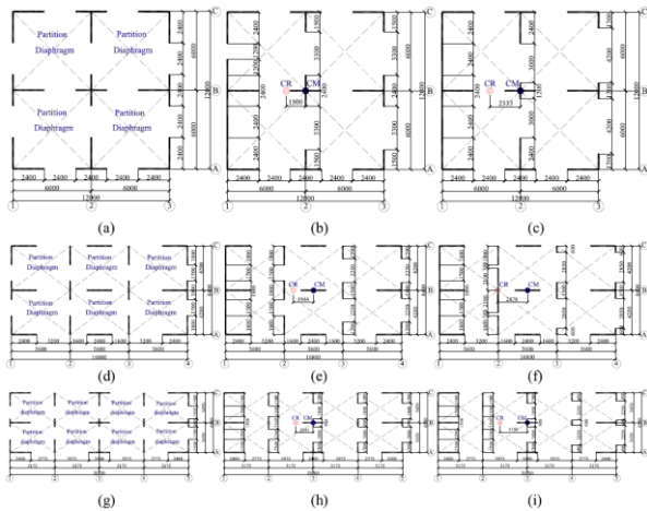
Figure 33: Three groups of single-storey baseline houses with different bracing wall layouts [68].
