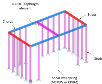
Figure 34: Timber3D model for test building [42].
