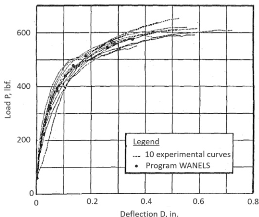
Figure 21: Comparison between the simulation results of program WANELS and ten experimental results on a wall only sheathed by plasterboards on one side [56].
