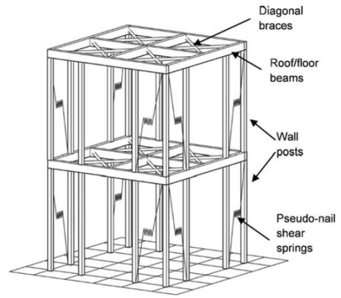
Figure 30: Schematics of a "PB3D" model [66].
