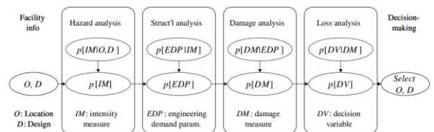
Figure 41: Seismic loss estimation framework proposed by PEER [80].
