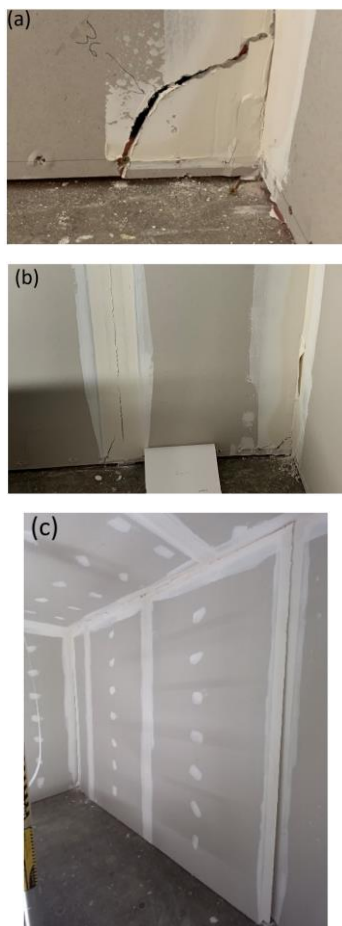
Figure 45: Damage observations of the test structure [88]: (a) local plasterboard damage; (b) failure of vertical sheet joints of plasterboard; (c) out-of-plane buckling of plasterboard.
