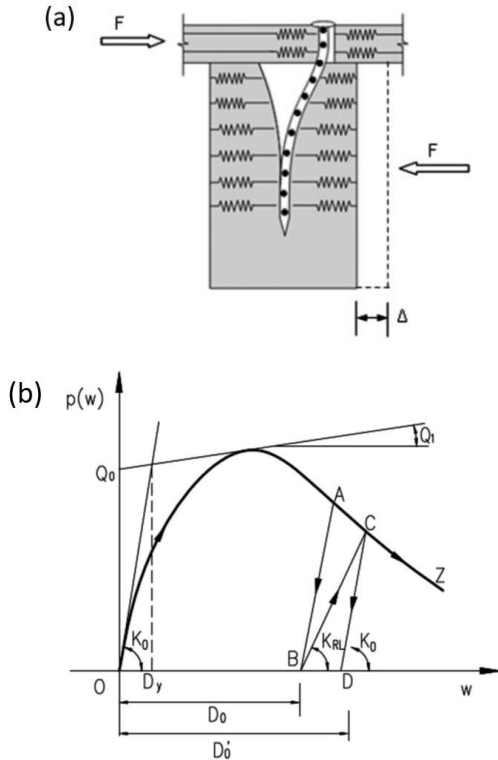
Figure 29: HYST algorithm: (a) schematics of HYST panel-frame nailed connection; (b) loading and unloading of wood medium in modified HYST algorithm [48].
