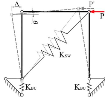
Figure 27: A modified macro element model [65].
