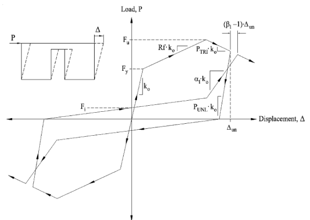
Figure 28: Stewart's hysteresis model [50].
