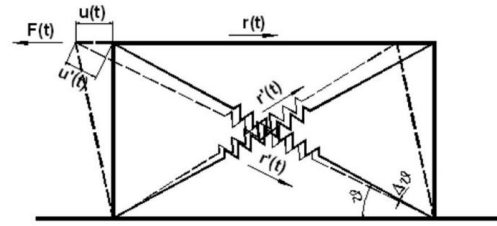
(b) Racking of Diagonal-Spring Shear Wall Model
