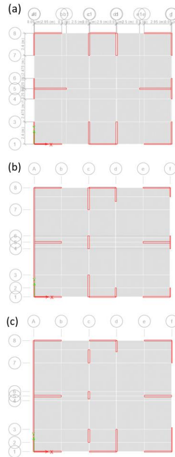
Figure 32: Floor plans of single-storey rectangular case study houses [67]: (a) regular; (b) 50% irregularity; and (c) 100% irregularity.
