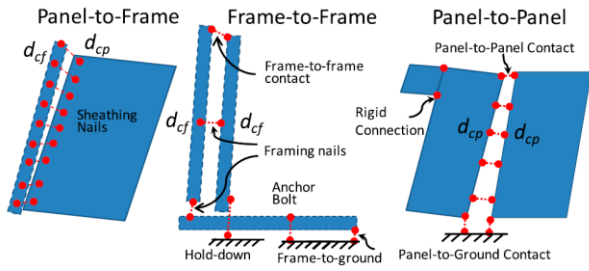
Figure 24: Connection elements of the detailed model [61].
