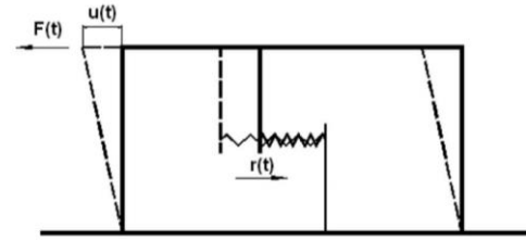
(a) Single-Spring Shear Wall Model
