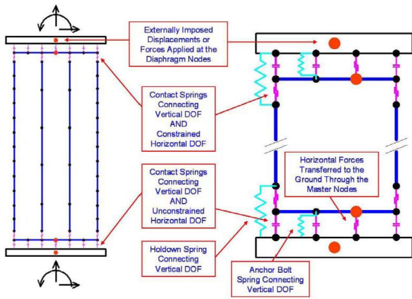
Figure 25: Detailed numerical model of the framing domain [63].
