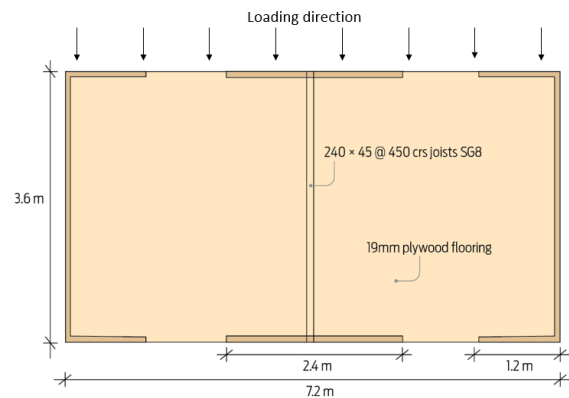
Figure 44: Floor plan of the test structure [88].
