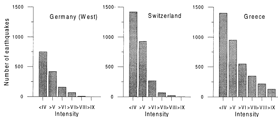
Figure 1 Histograms of the intensities in three European Countries
