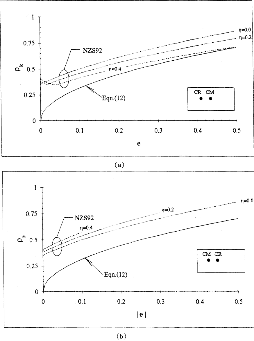
Figure 13 Minimum torsional stiffness to satisfy the edge displacement criterion
